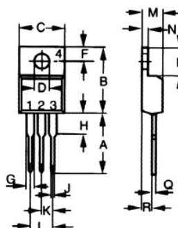
TO-220AB
